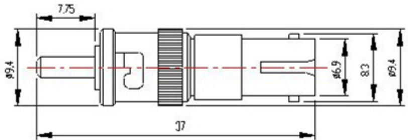
ST/PC Plug Type Fixed Attenuator
