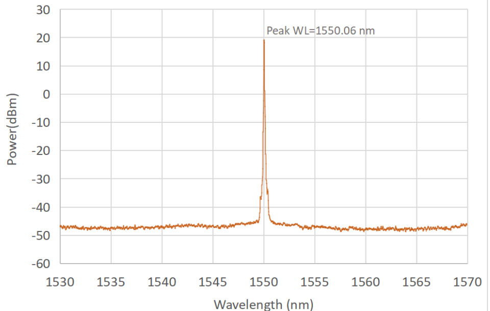
Optical Spectrum of 1550nm Laser Source
